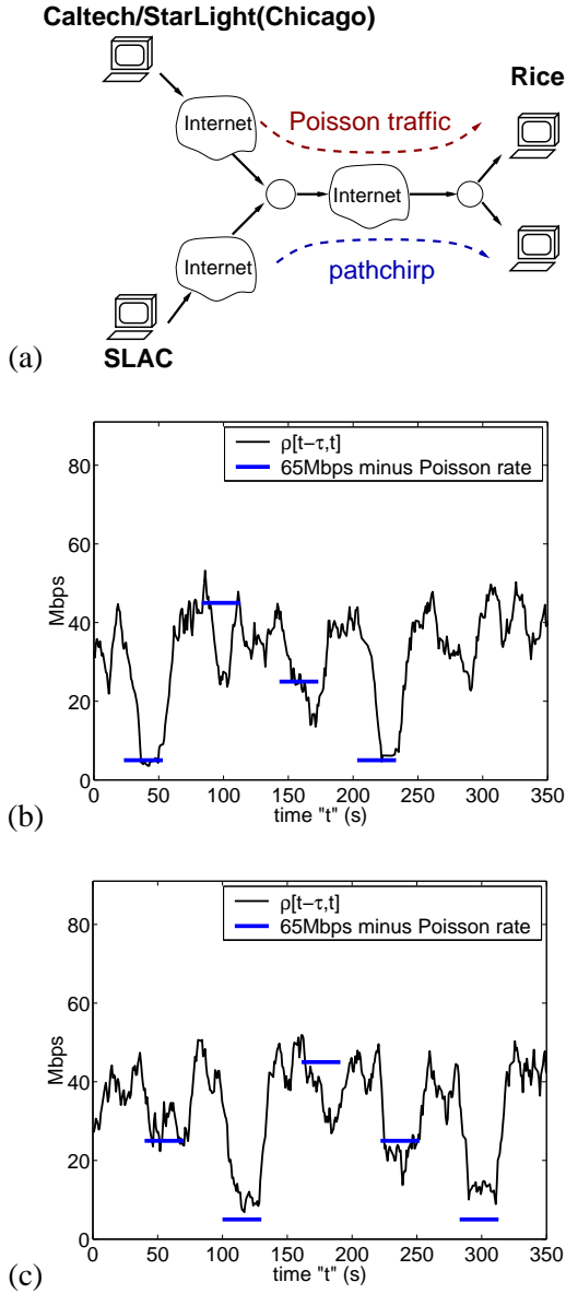
Fig. 14. (a) Setup for the Internet experiment. (b) Available bandwidth estimates when Poisson traffic originates at Caltech. (c) Available bandwidth estimates when Poisson traffic originates at StarLight (Chicago). Observe that the pathChirp estimates fall in proportion to the introduced Poisson traffic.
